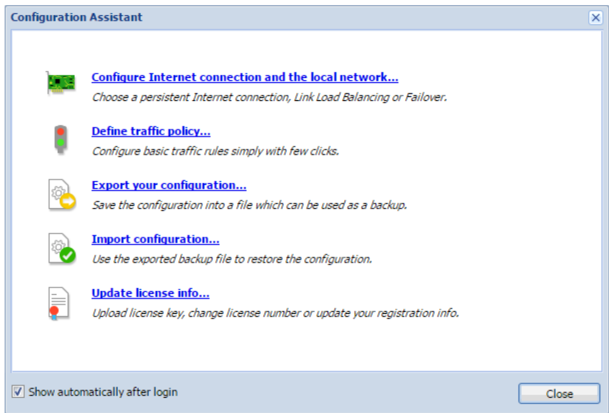
Figure 1 Configuration Assistant
