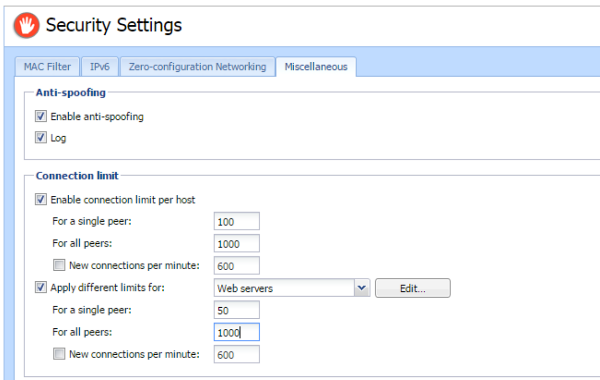
Figure 1 Connection limits
