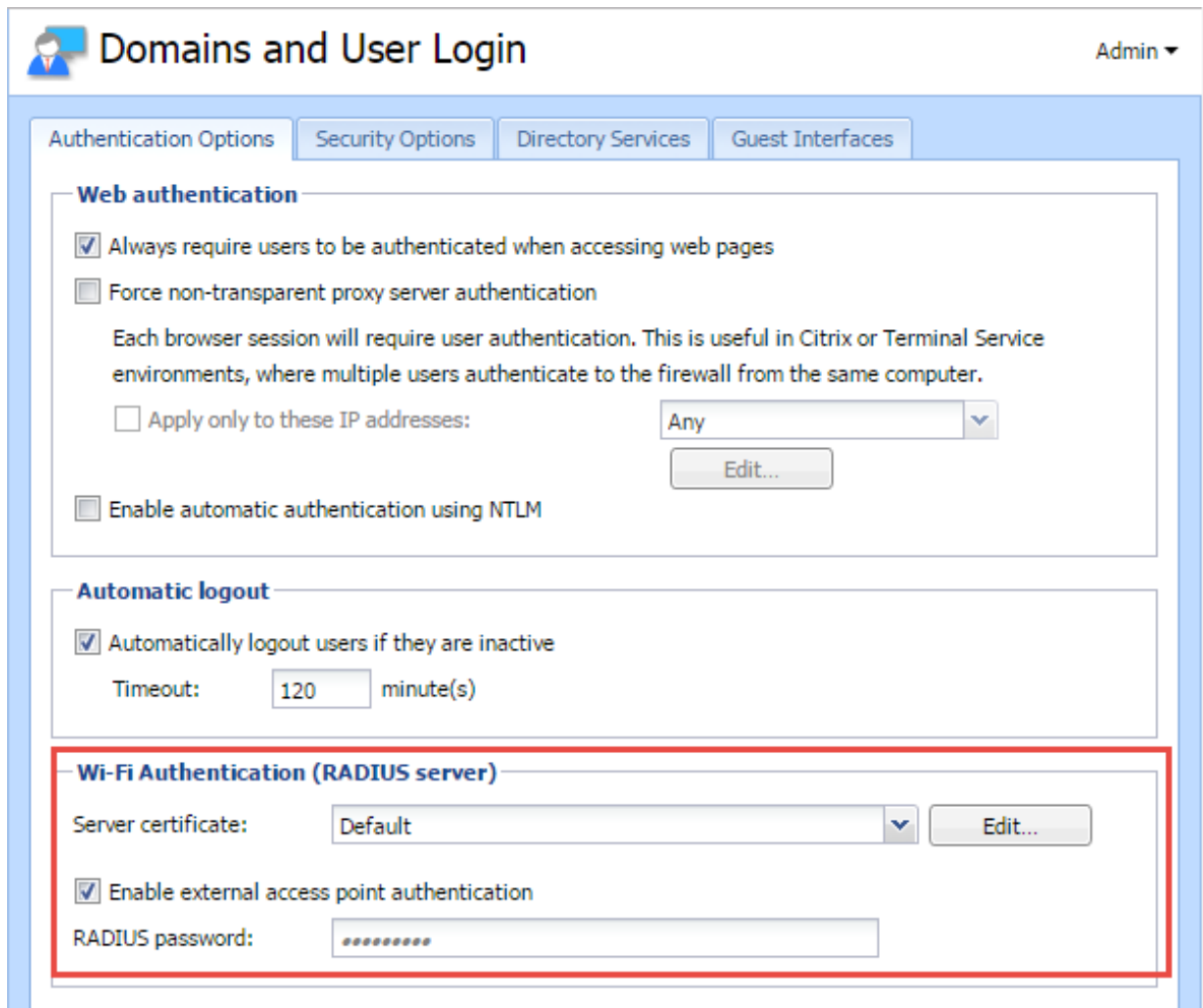
Figure 1 Wi-Fi Authentication
