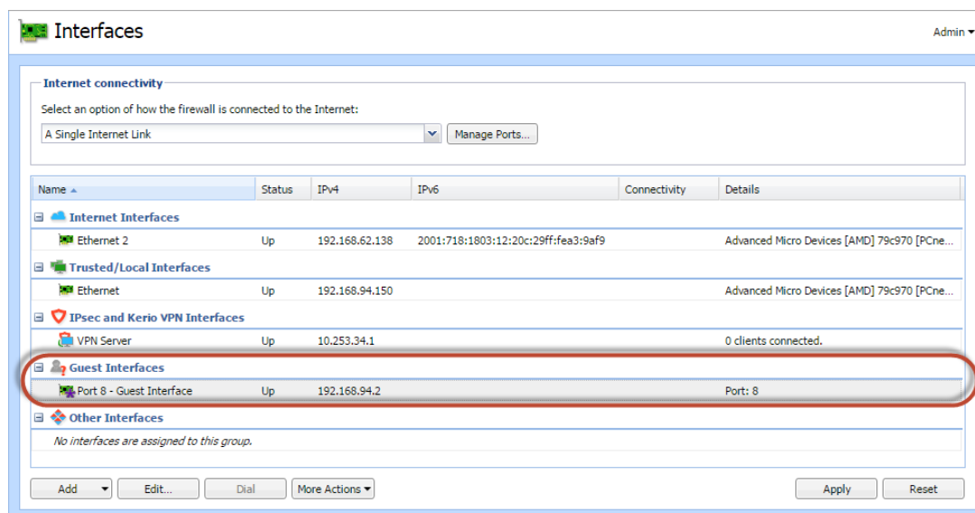
Figure 1 Section Interfaces
