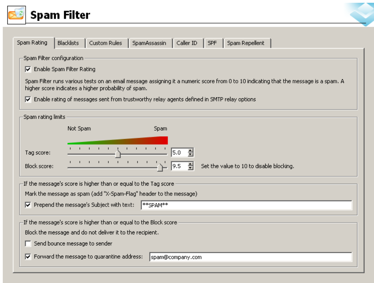
Figure 13.1 Spam Rating tab
