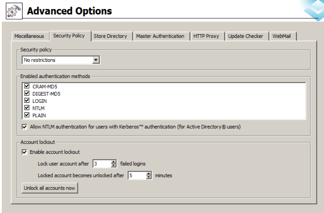
Figure 28.2 Enabling the Allow NTLM authentication for users with Kerberos authentication option
