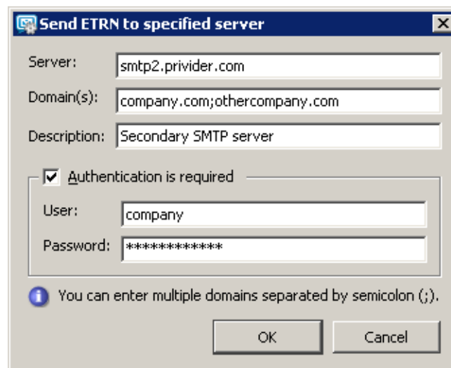
Figure 12.14 Setting parameters for accessing the server
