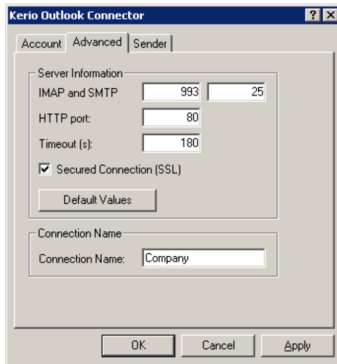
Figure 33.13 Account settings — ports
