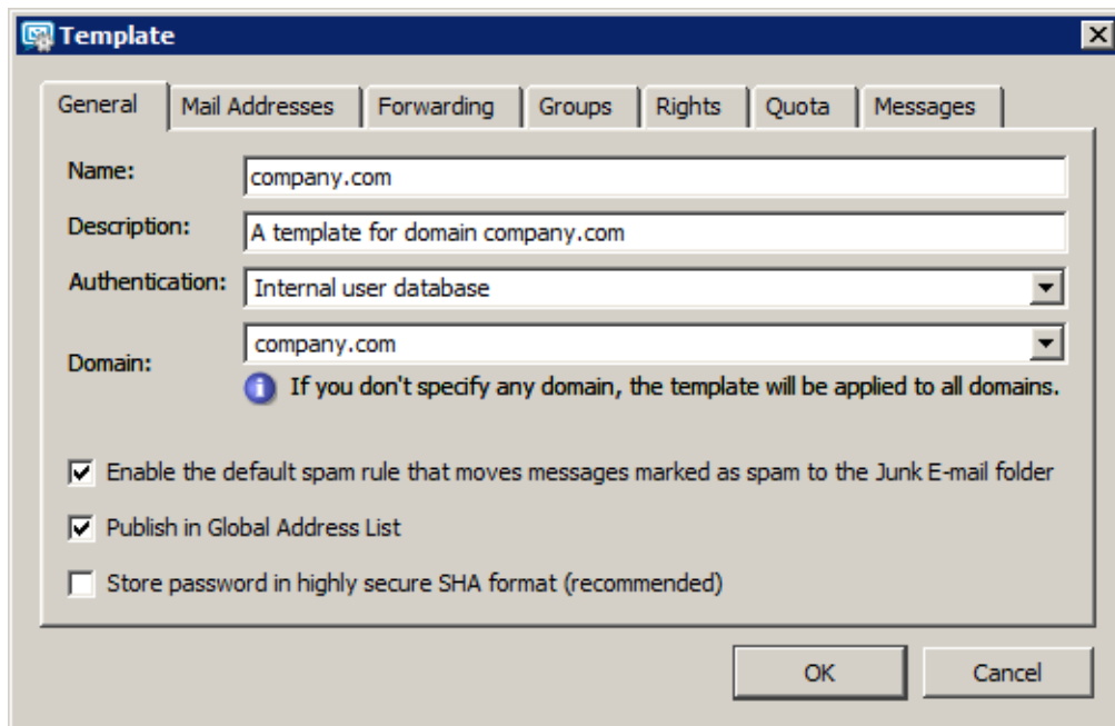
Figure 8.23 Defining a template
