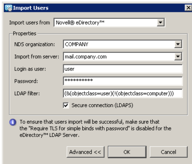
Figure 8.21 Import users from Novell eDirectory
