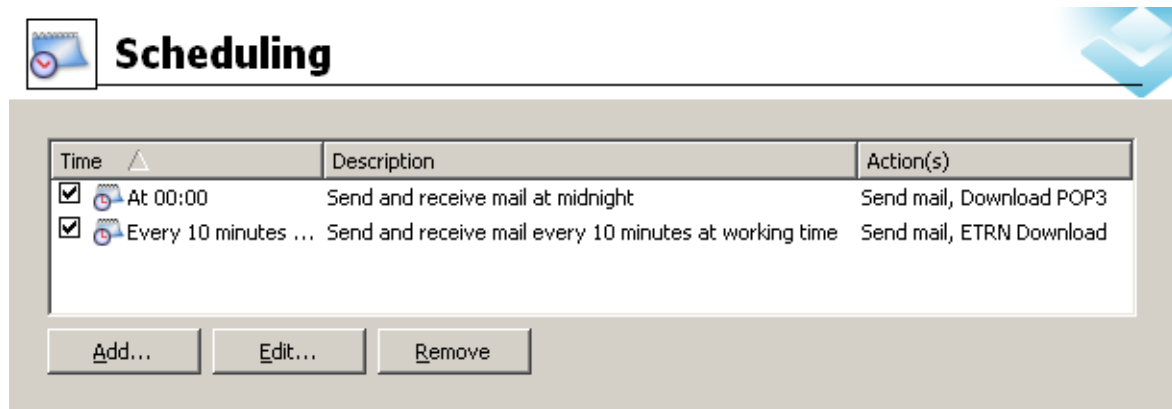
Figure 20.1 Scheduling
