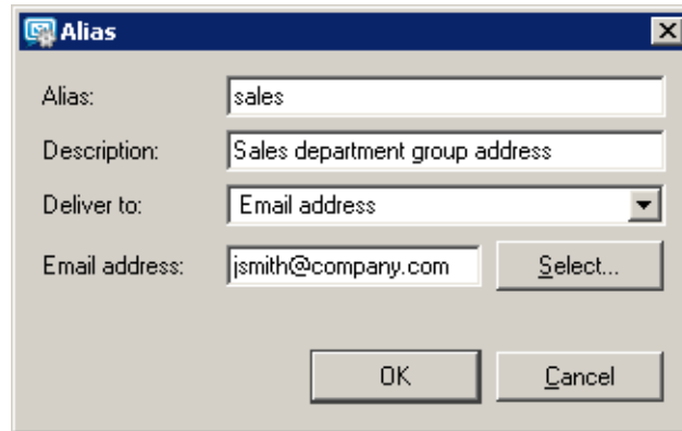
Figure 12.6 Defining Alias
