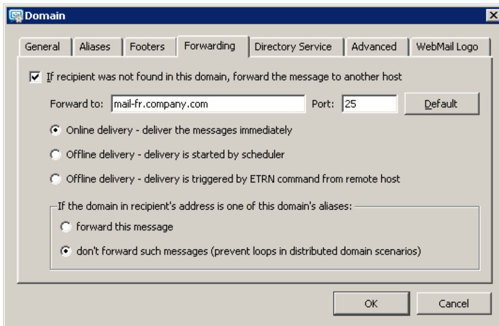
Figure 7.10 Forwarding settings
