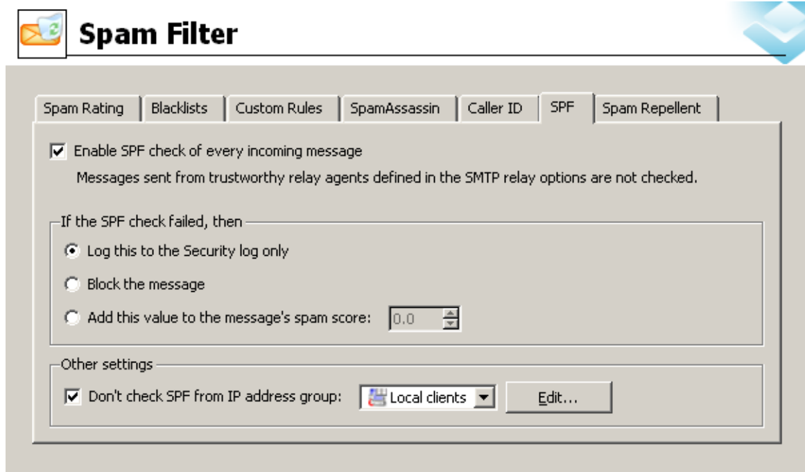
Figure 13.8 SPF
