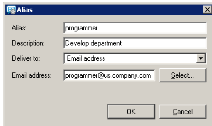
Figure 7.11 Alias settings
