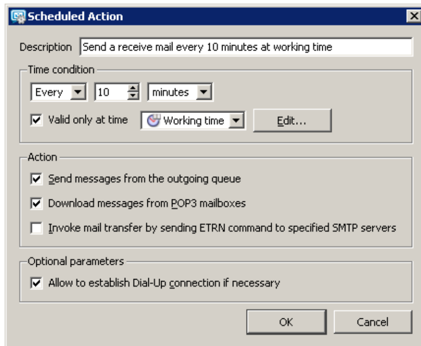
Figure 20.2 Scheduled Action
