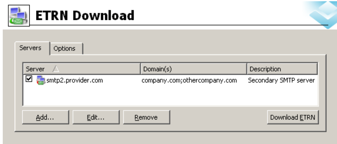
Figure 12.13 ETRN Download
