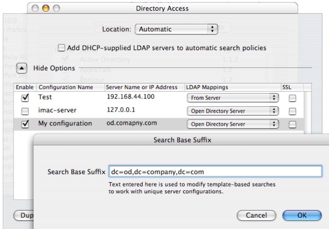
Figure 27.8 Directory Access — configuration of the Open Directory server
