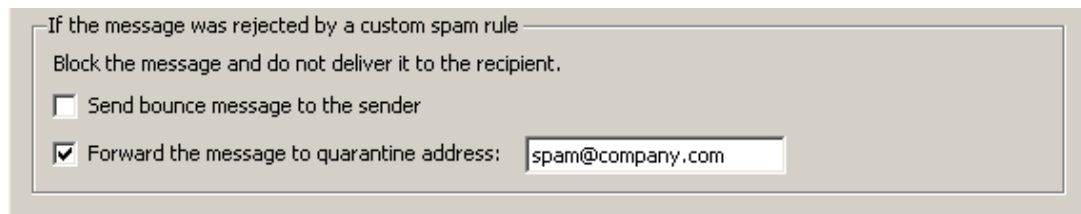
Figure 13.10 Forward the message to quarantine address
