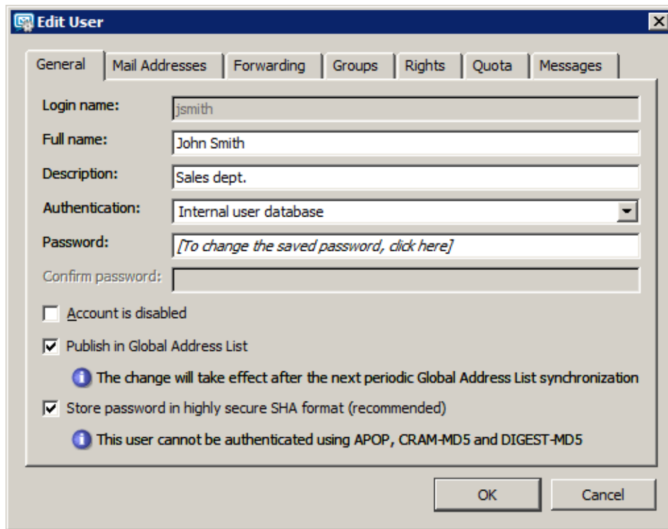
Figure 8.10 Editing User Account
