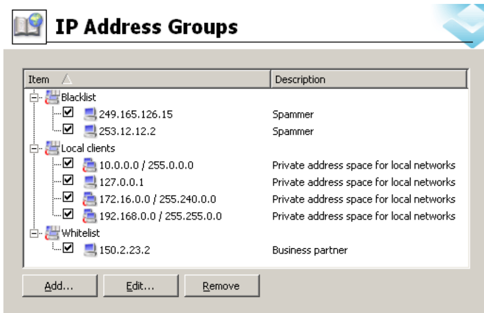
Figure 19.1 IP Address Groups
