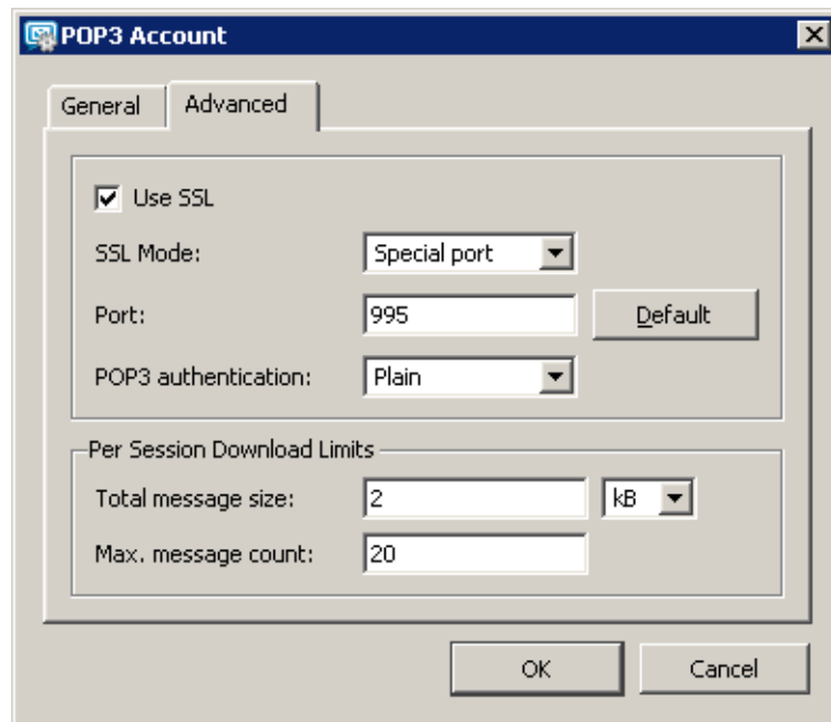
Figure 12.10 More detailed settings for downloading POP3 mailboxes
