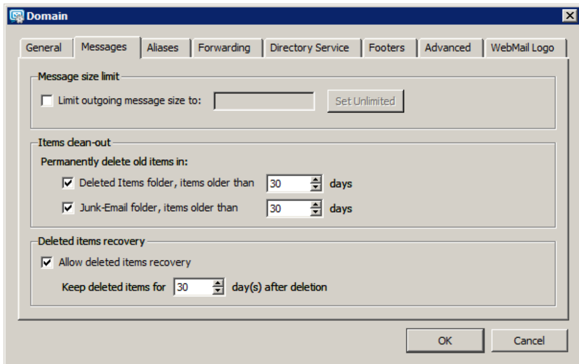
Figure 7.5 Domain Settings — Messages
