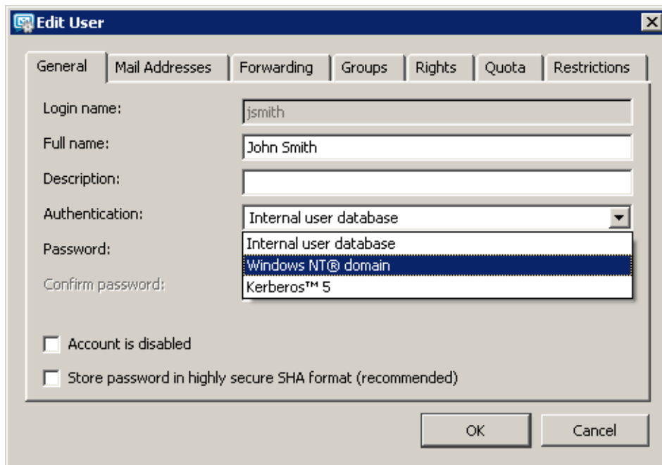
Figure 28.3 User authentication settings
