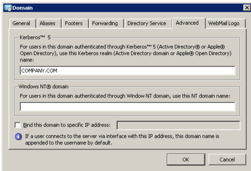
Figure 27.1 Setting the Active Directory domain in Kerio MailServer
