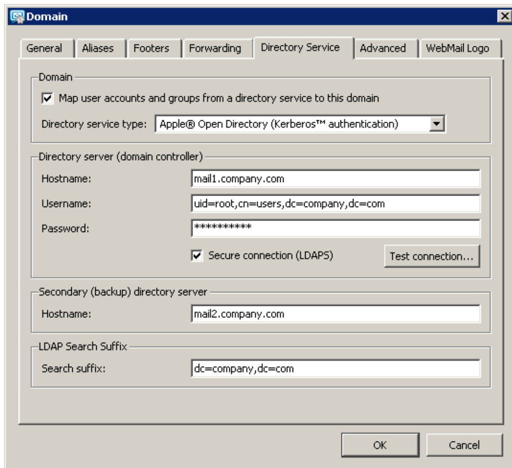
Figure 10.6 Domain settings — Apple Open Directory
