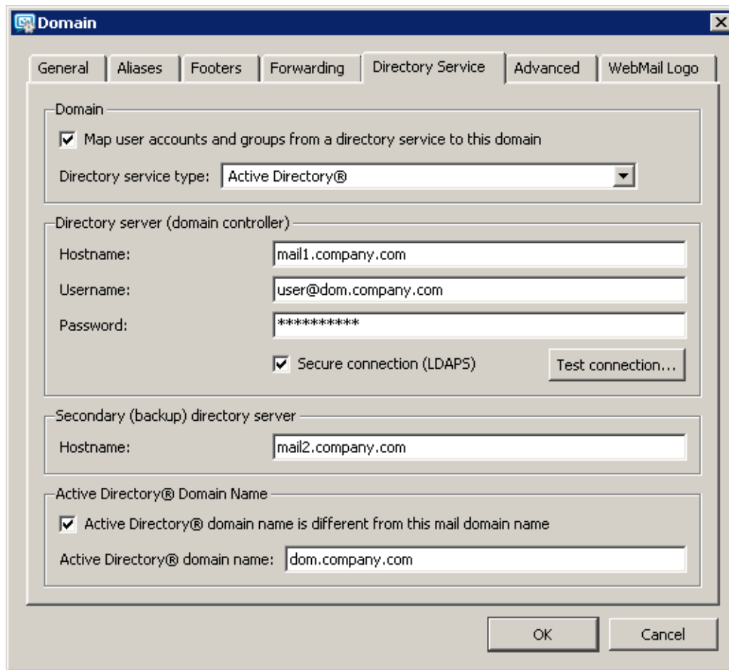
Figure 10.1 Domain settings — Active Directory
