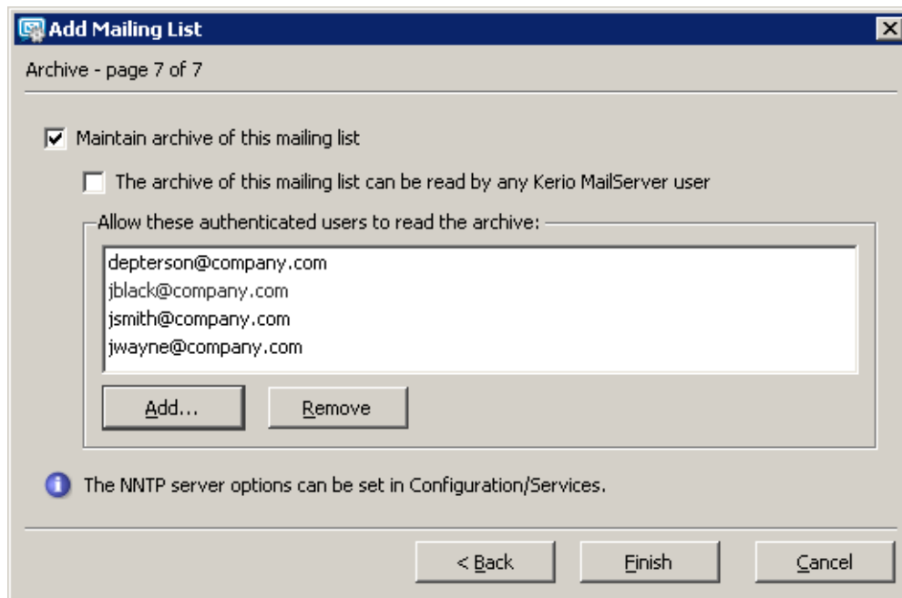
Figure 22.9 Creating a mailing list — maintain archiving
