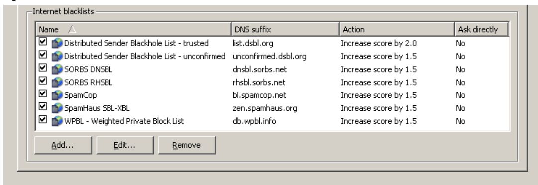
Figure 13.3 Internet databases
