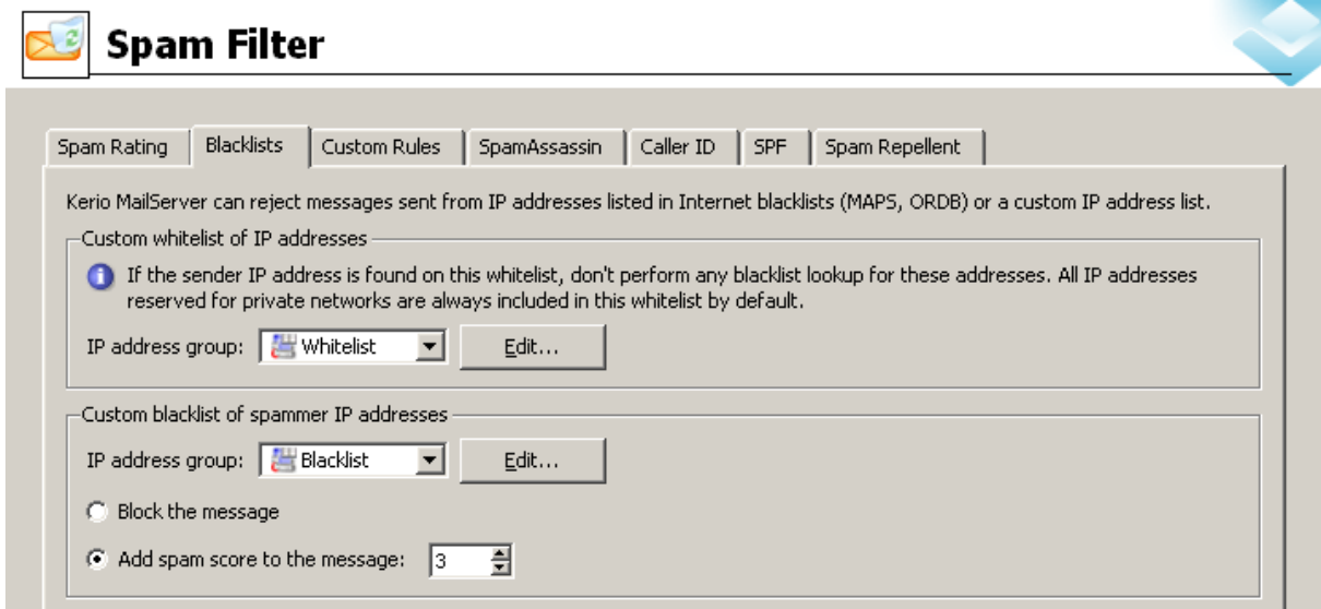
Figure 13.2 Blacklists tab
