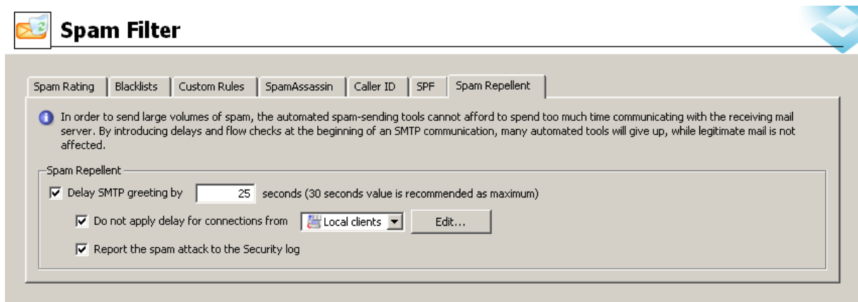
Figure 13.9 Spam repellent
