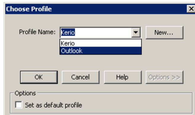
Figure 33.15 Choose Profile
