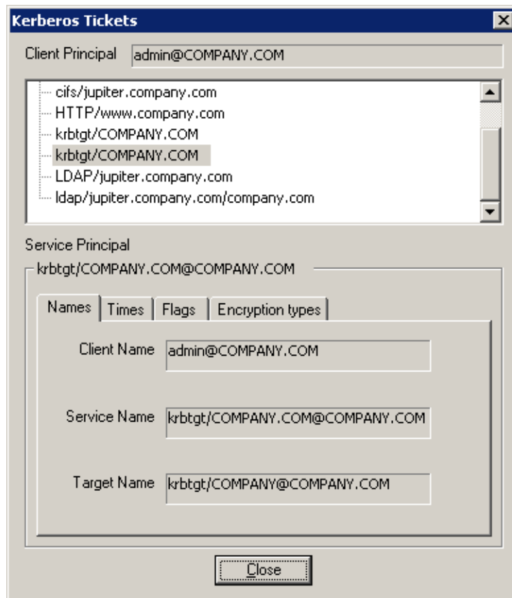
Figure 27.2 Kerberos tickets displayed in Kerbray
