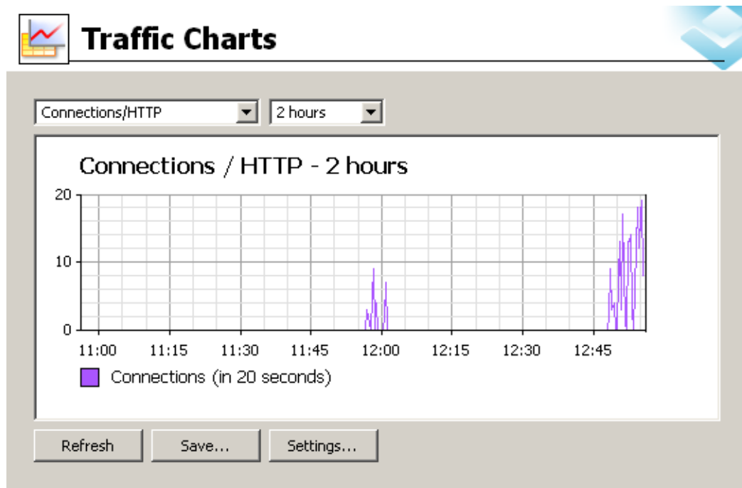
Figure 24.6 Traffic Charts
