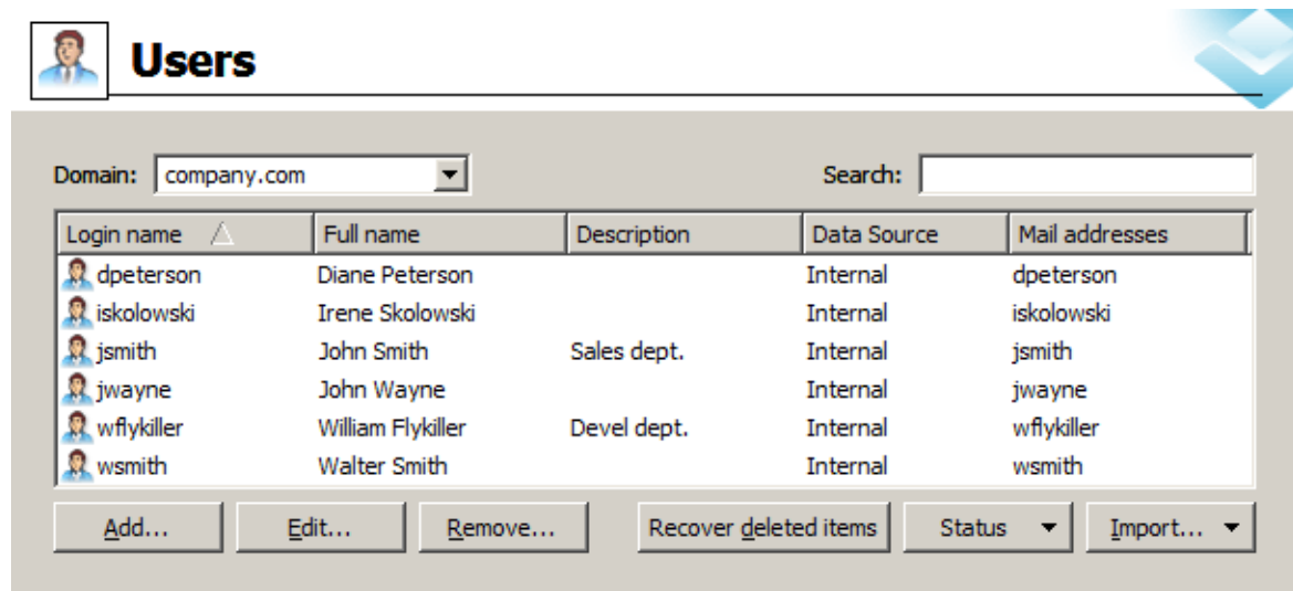
Figure 8.1 Users
