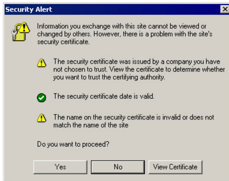
Figure 16.1 Security Alert
