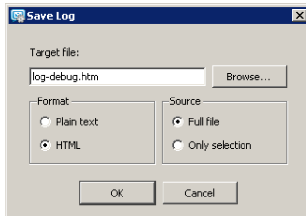
Figure 25.2 Save log
