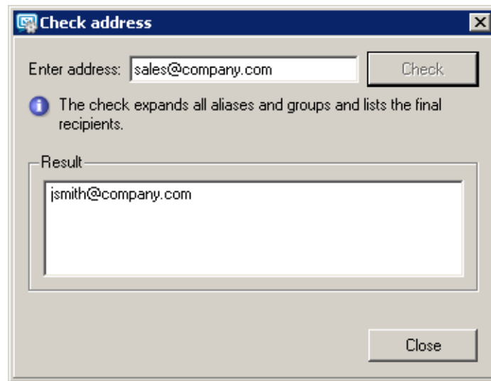
Figure 12.7 Check Address
