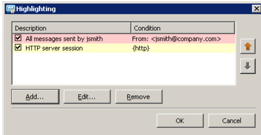
Figure 25.4 Highlighting
