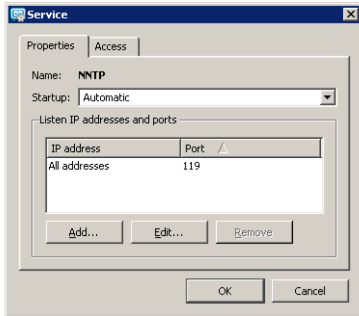
Figure 6.2 Service Parameters
