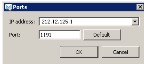
Figure 6.3 Ports
