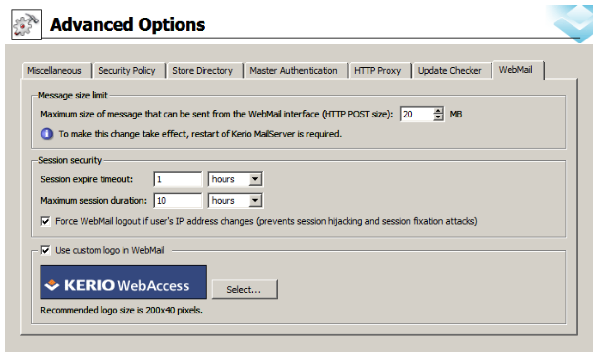
Figure 17.4 Securing of the connection between the server and the Kerio WebMail interface
