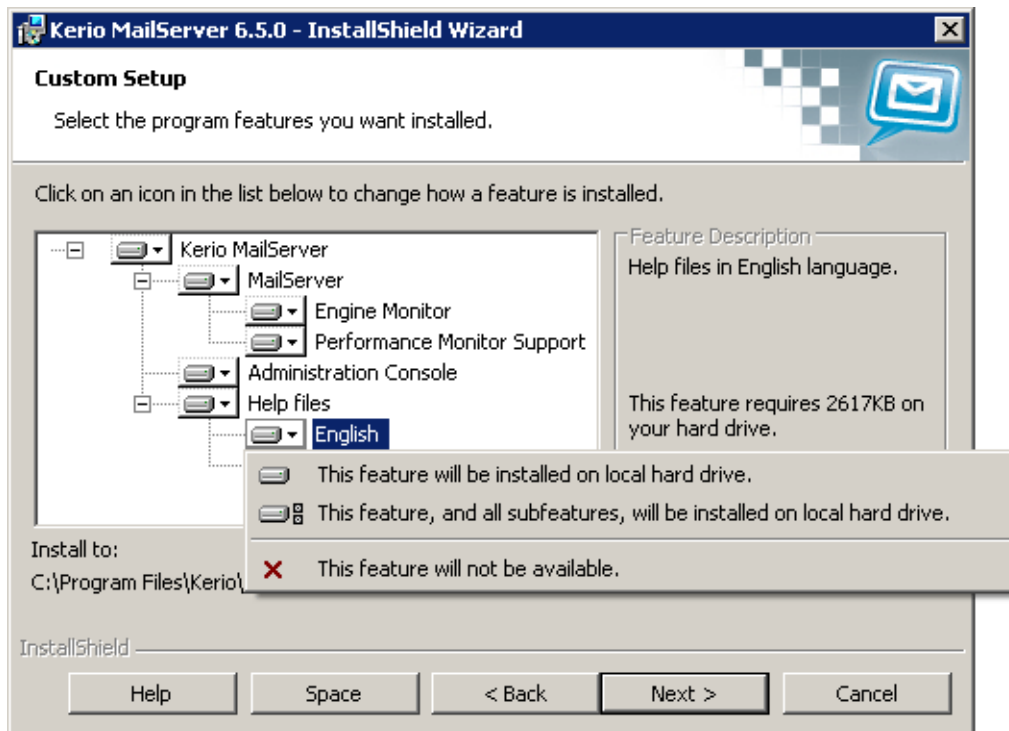
Figure 2.1 Custom installation
