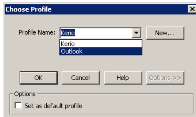
Figure 33.15 Choose Profile
