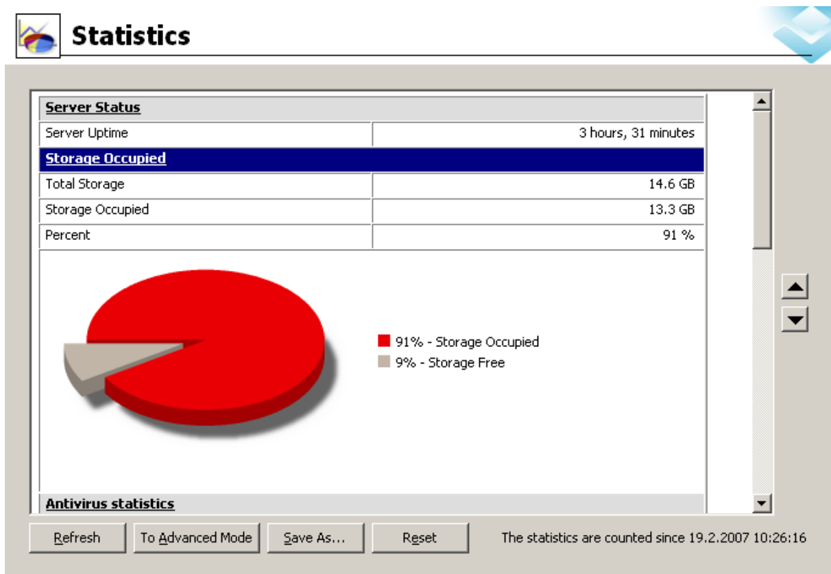
Figure 24.8 Statistics
