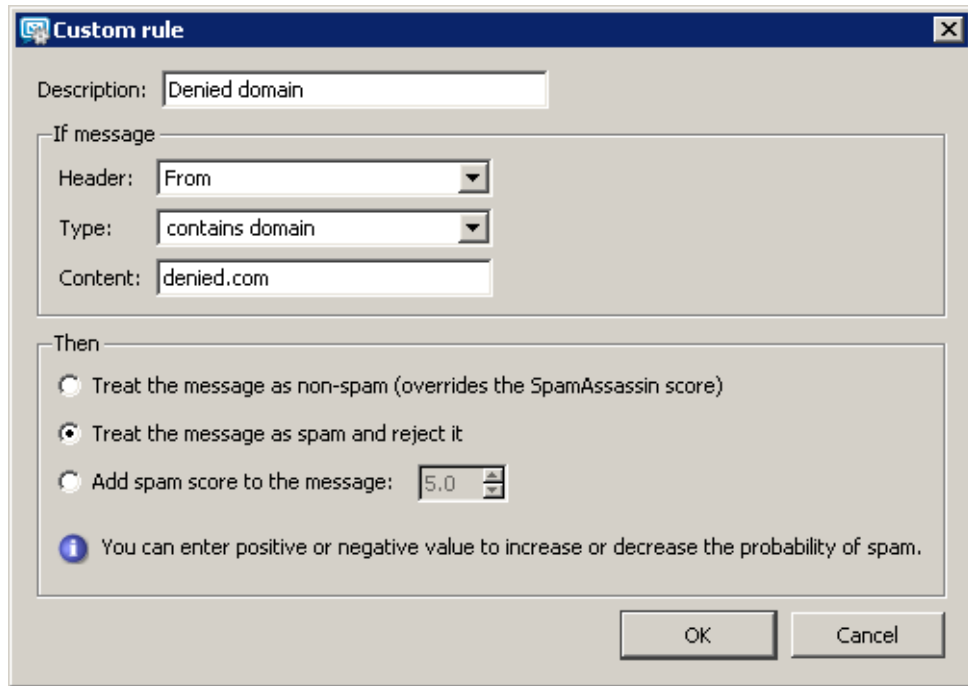
Figure 13.6 Defining rule
