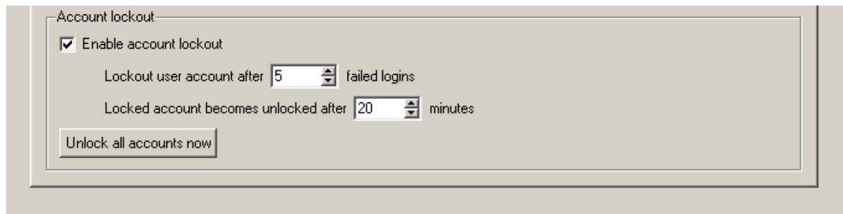
Figure 12.17 Account lockout
