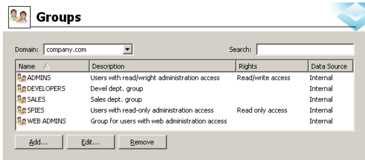
Figure 9.1 Groups
