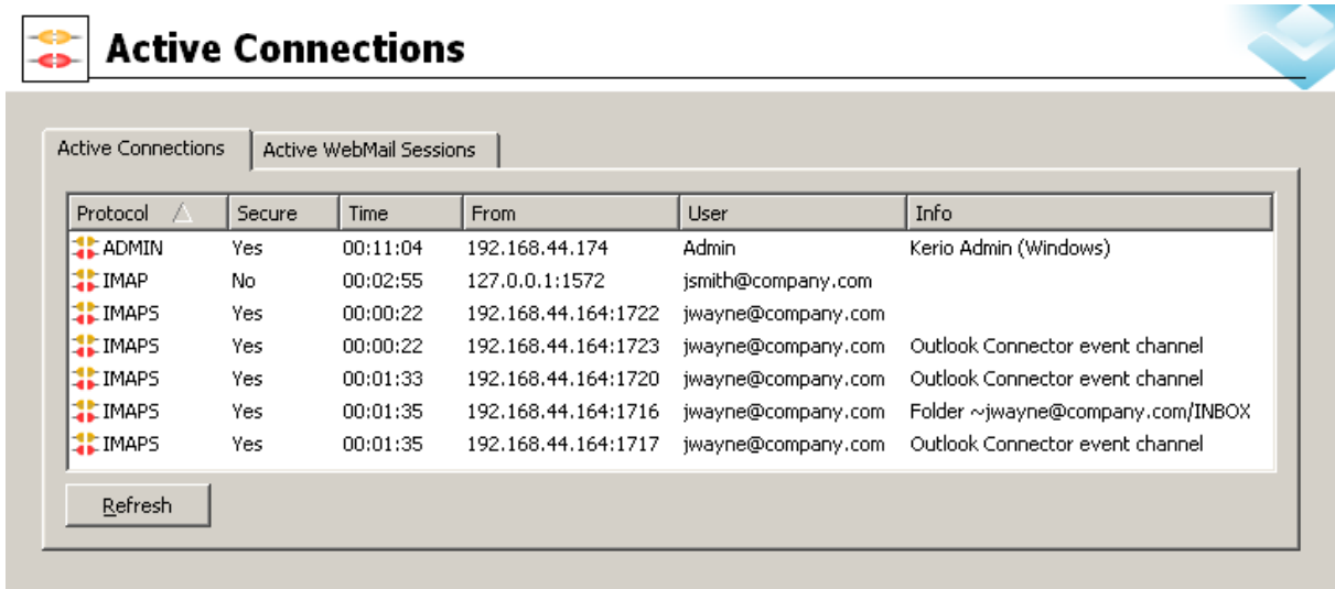
Figure 24.3 Active Connections
