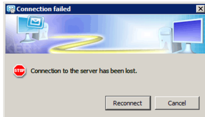
Figure 5.3 Reconnecting
