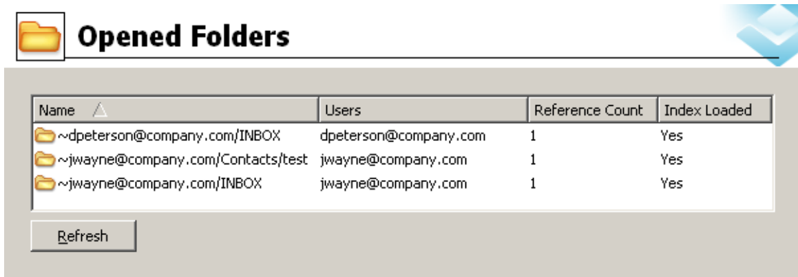
Figure 24.5 Opened Folders
