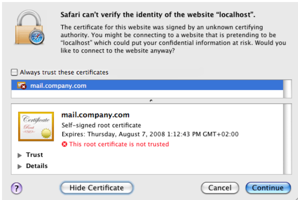
Figure 16.5 Certificate Details
