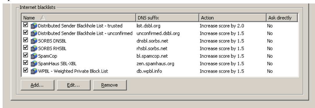
Figure 13.3 Internet databases
