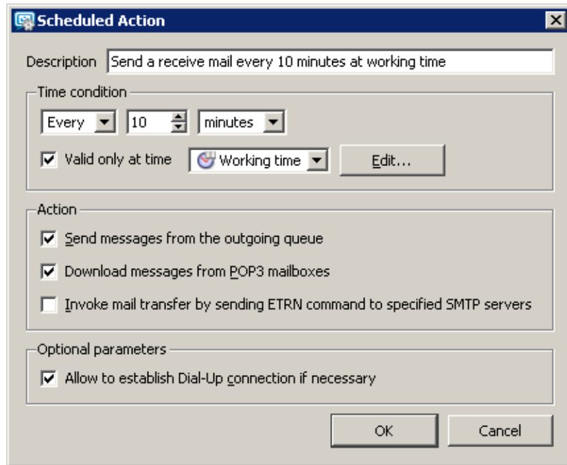
Figure 20.2 Scheduled Action
